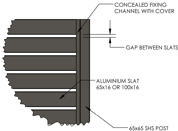
FENCE DETAILS
